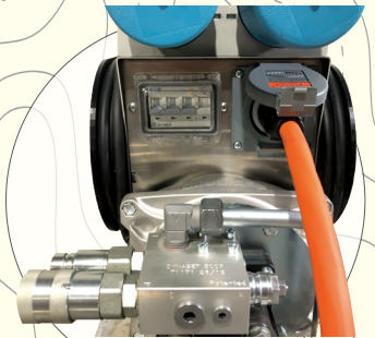
13mm (1/2") Flush Face QD (DHP Circuit)
